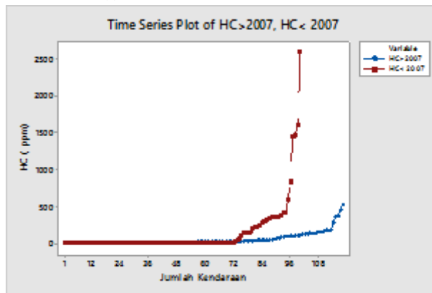
Gambar 7. Time Plot of HC > 2007 dan HC < 2007
